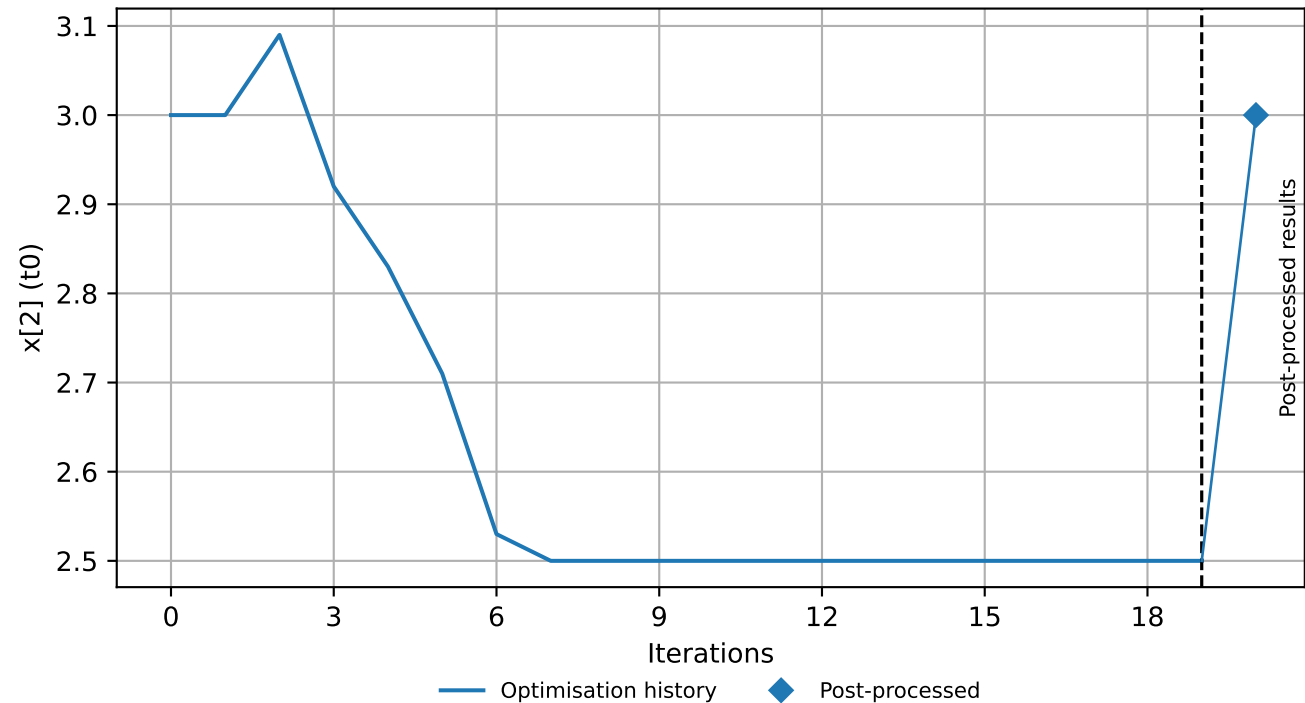
SLP Design variable convergence: t0
